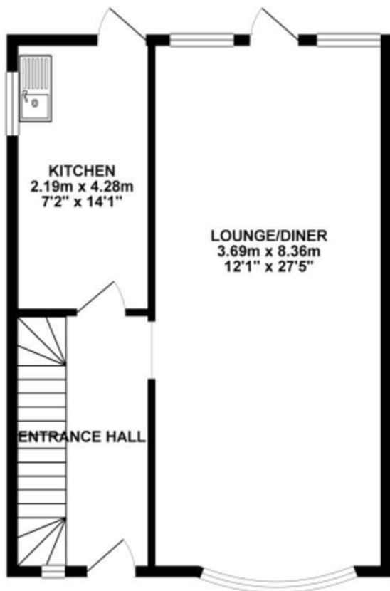
GROUND FLOOR 28.8 sq. m. ( 310.00 sq. ft. )
